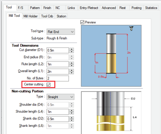
Center Cutting Tool Recognition
